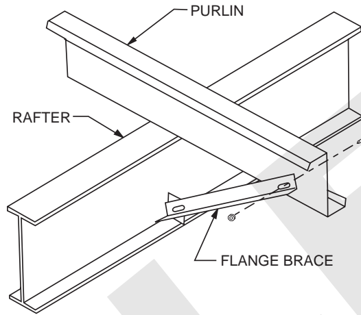
FB FLANGE BRACE CONNECTION
